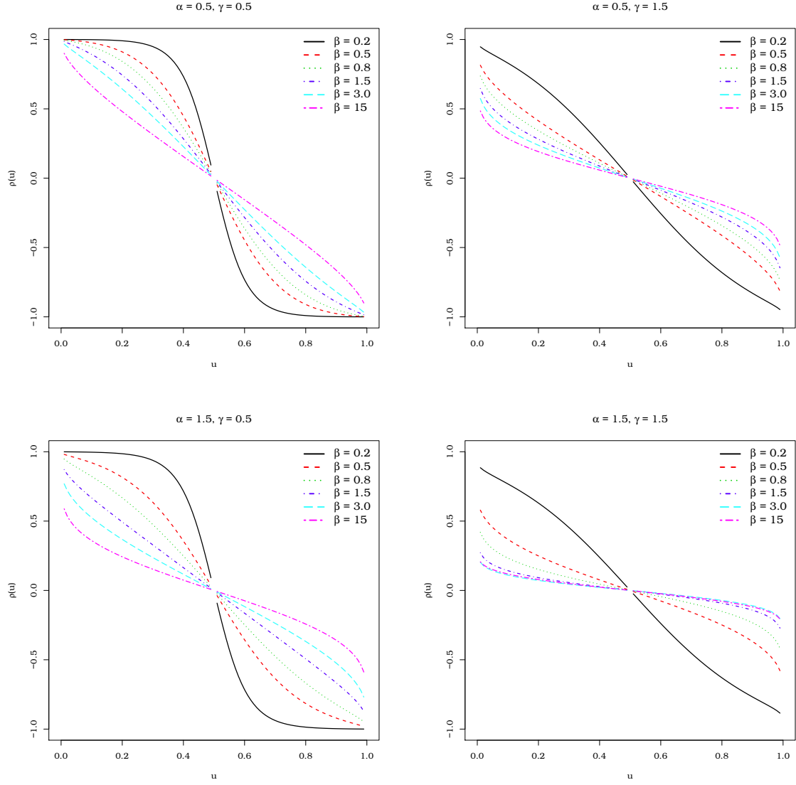
Figure 2.3: The MacGillivray's skewness of the EGPW distribution.
