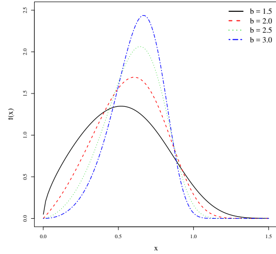
(b) a = 1.5, \alpha = 2 and \lambda = 0.4
