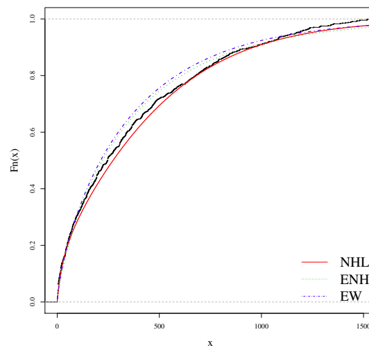
Figure 3.5: Estimated cdfs of the NHL, ENH and EW models for the reinfection times.
