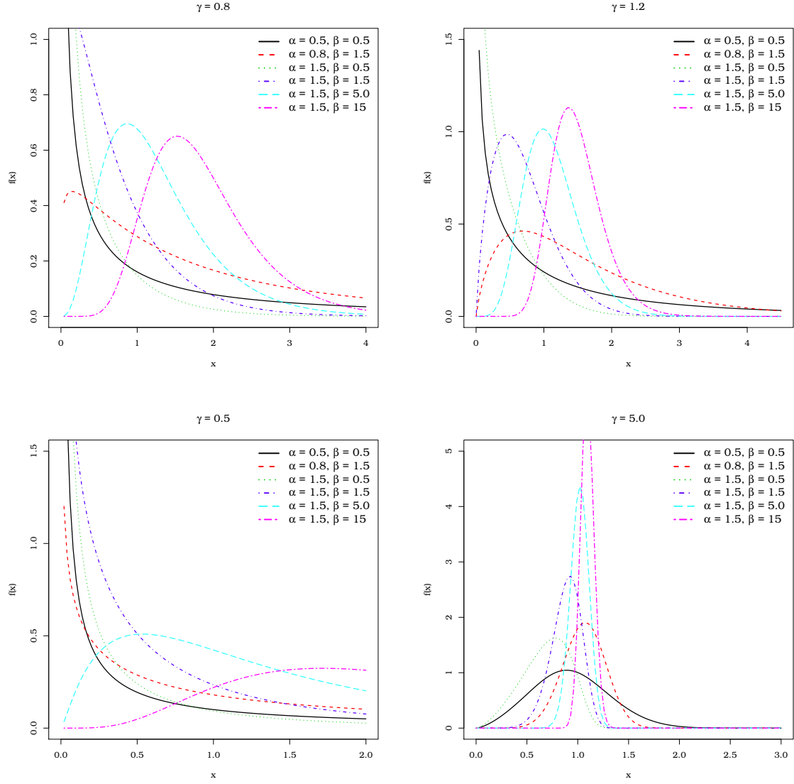
Figure 2.1: Plots of the EGPW density for \lambda = 1 .
