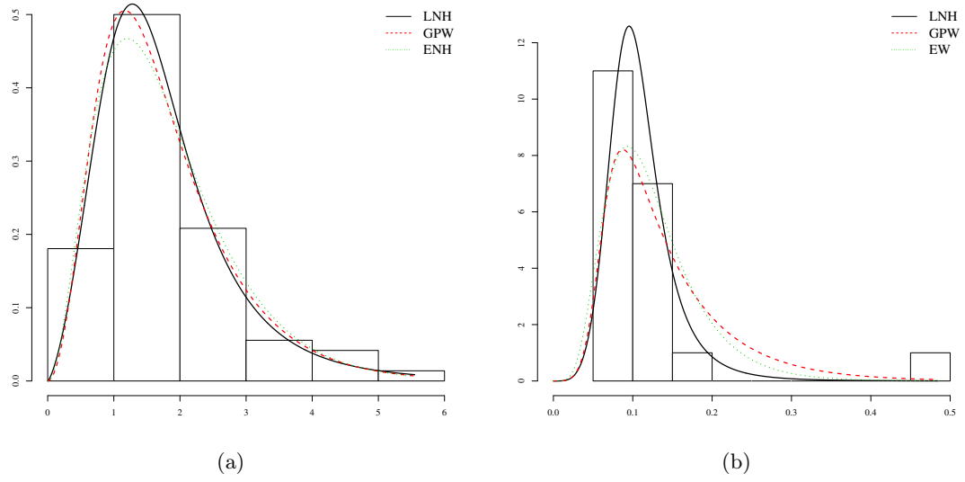
Figure 5.4: Histogram and estimated densities of the (a) LNH, GPW and ENH models for the guinea pigs data set; (b) LNH, GPW and EW models for the mechanical components data set.
