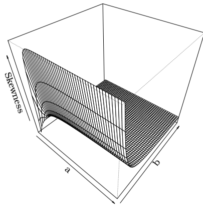
(a) \alpha = 1.5, \lambda = 1.5
