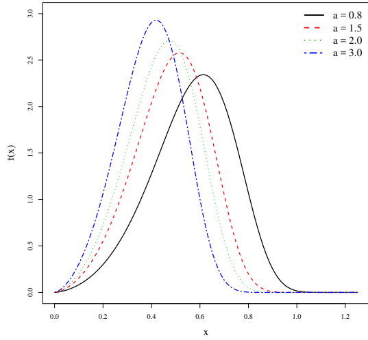
(a) b = 2.5, \alpha = 2 and \lambda = 0.5
