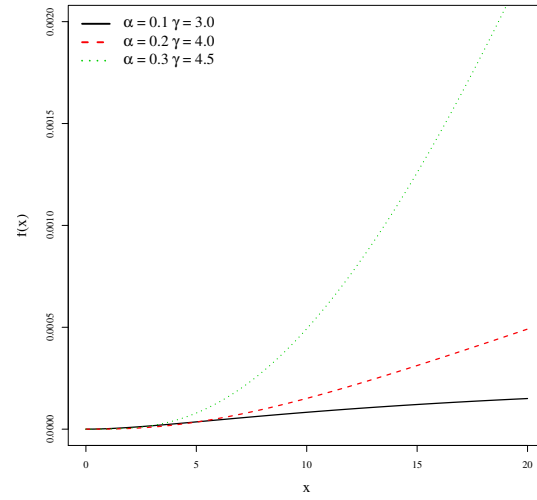
(b) For \lambda = 0.1
