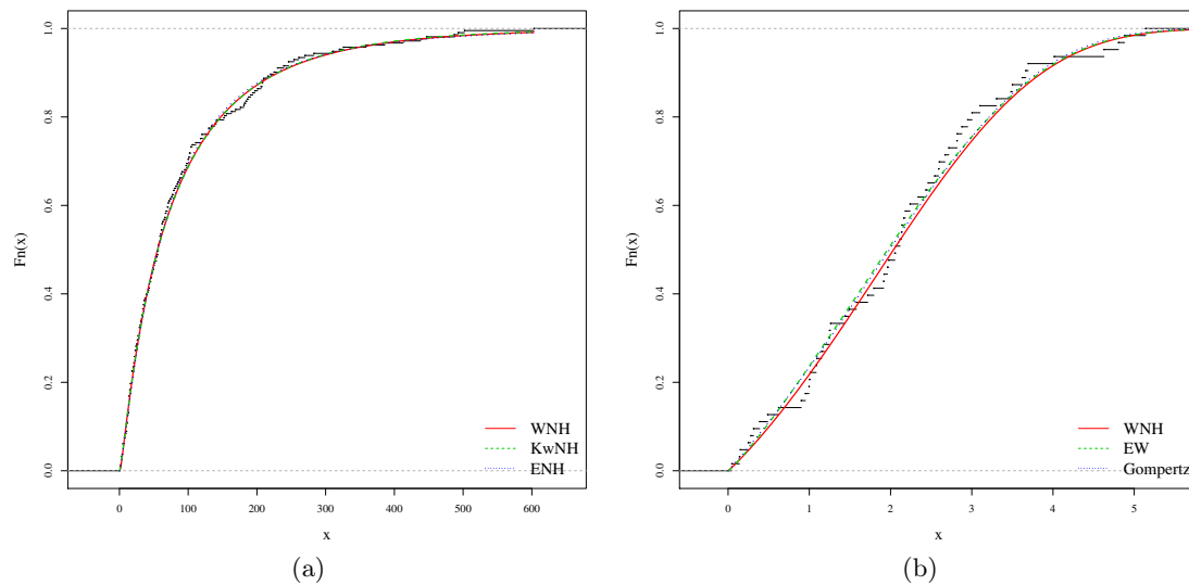
Figure 4.6: Estimated and empirical cdfs of the (a) WNH, KwNH and ENH models for the Boeing 720 data set; (b) WNH, EW and Gompertz models for the Aircraft Windshield data set
