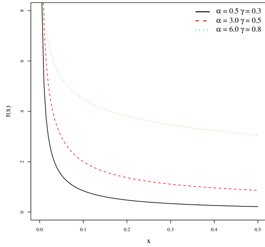
(a) For \lambda = 1
