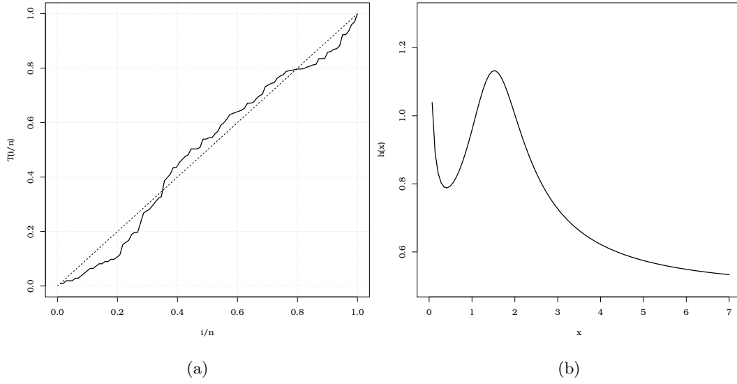
Figure 2.4: The TTT plot and EGPW hrf for the stress-rupture failure times data.
