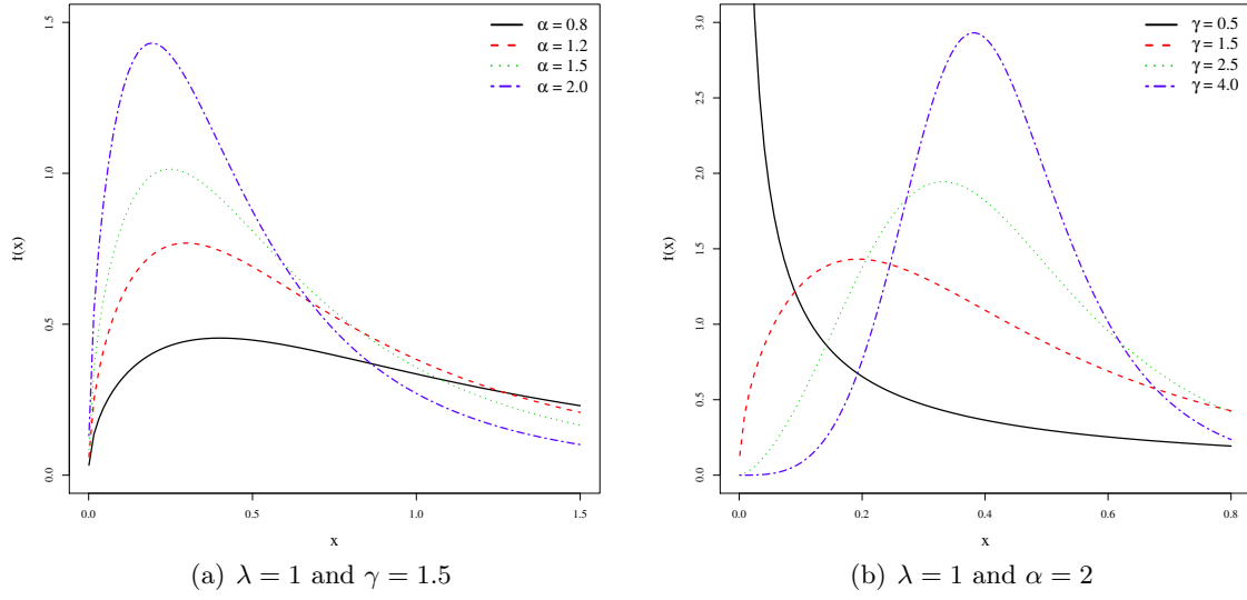
Figure 5.1: Plots of the LNH density.
