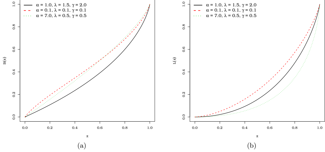
Figure 3.4: (a) Bonferroni curves for the NHL distribution for some parameter values; (b) Lorenz curves for the NHL distribution for some parameter values
