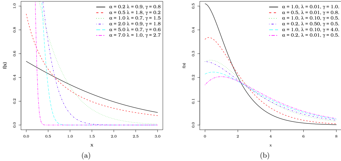
Figure 3.1: Pdf plots for the NHL distribution.
