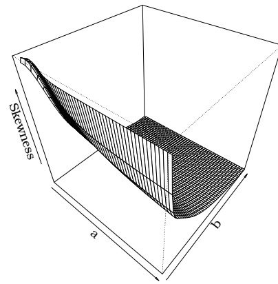
(b) \alpha = 0.1, \lambda = 1.5
