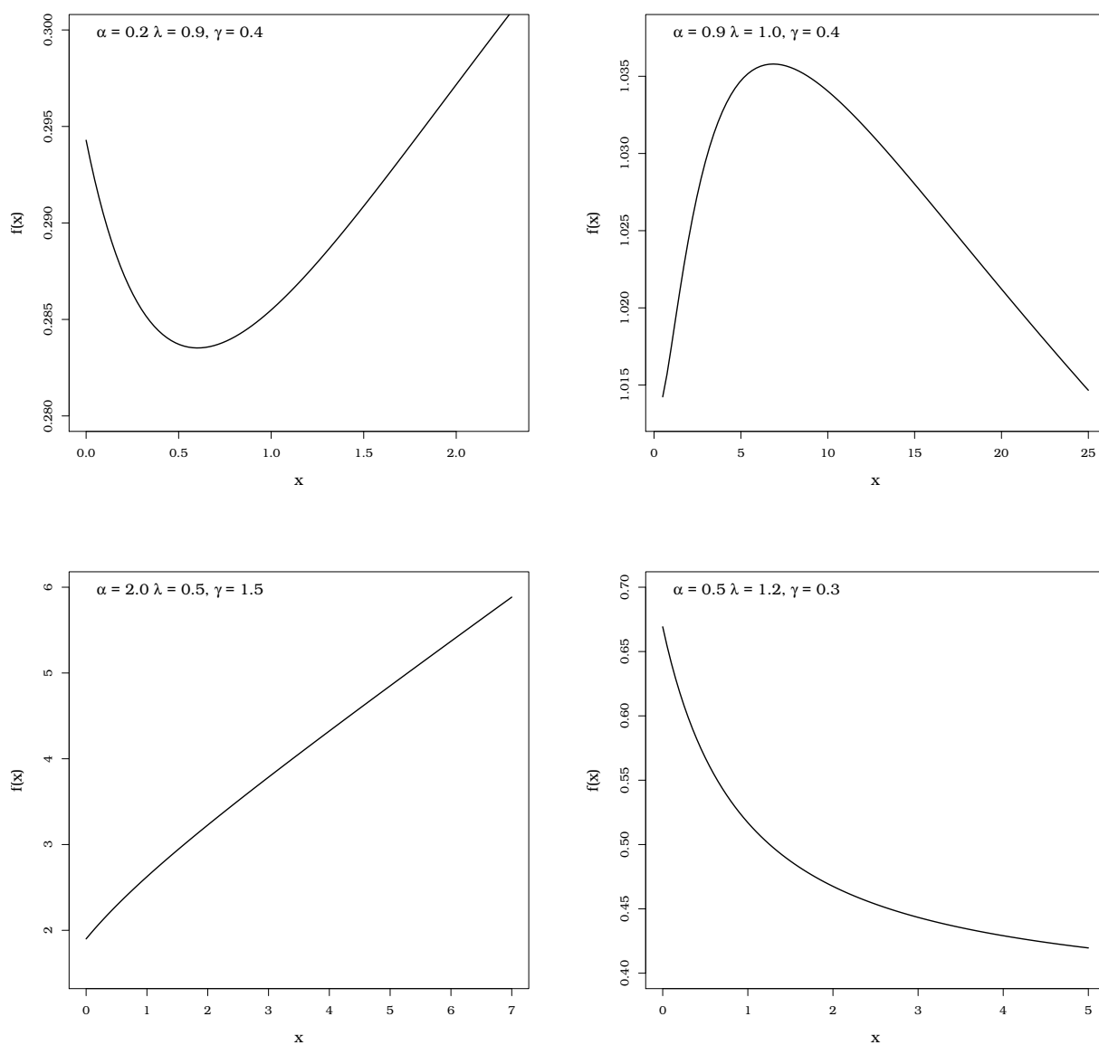
Figure 3.2: Hrf plots for the NHL distribution
