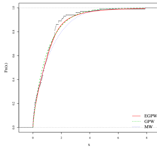
Figure 2.6: Estimated and empirical cdfs for EGPW, GPW and MW models for the stress-rupture failure times data.
