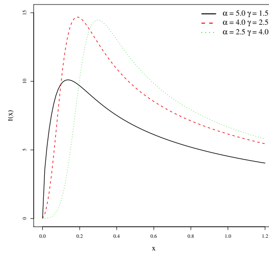
(c) For \lambda = 1.5
