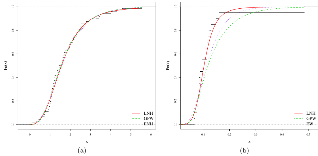
Figure 5.5: Estimated and empirical cdfs of the (a) LNH, GPW and ENH models for the guinea pigs data set; (b) LNH, GPW and EW models for the mechanical components data set.
