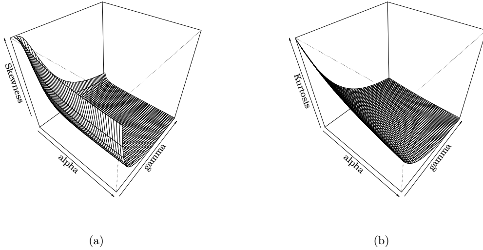
Figure 5.3: The Bowley skewness (a) and Moors kurtosis (b) of the LNH distribution.
