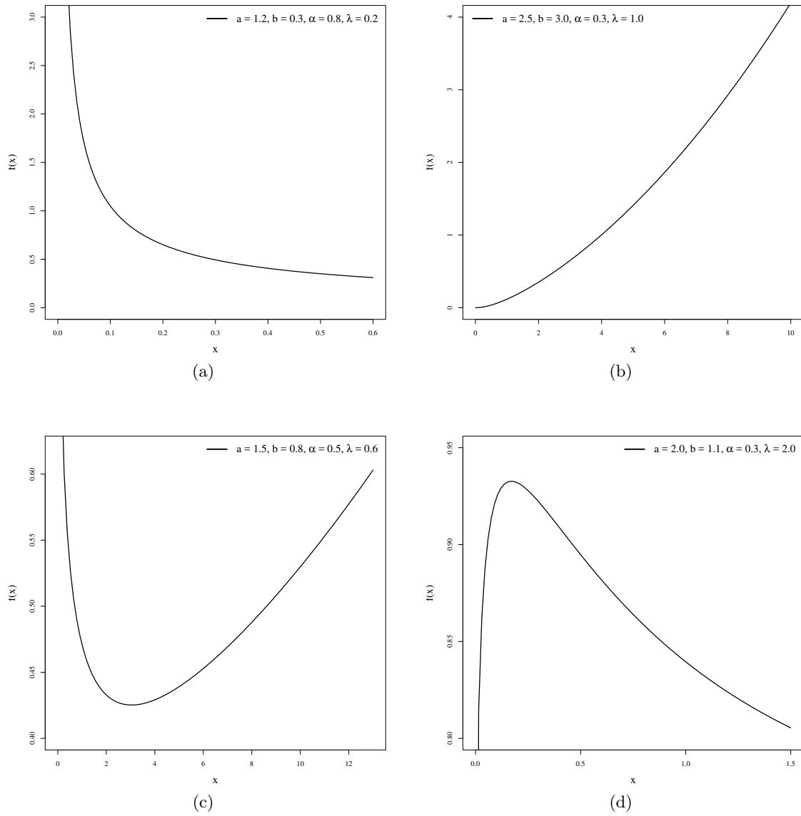
Figure 4.2: Plots of the WNH hrf.
