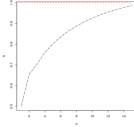
Figure 4.3: Sum of the coefficients S = \sum_{i,j=0}^n \omega_{i,j} of the linear combination in (4.7).
