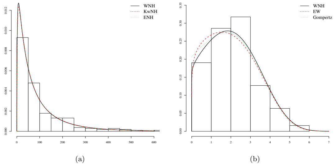
Figure 4.5: Histogram and estimated densities of the (a) WNH, KwNH and ENH models for the Boeing 720 data set; (b) WNH, EW and Gompertz models for the Aircraft Windshield data set
