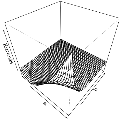
(c) \alpha = 1.5, \lambda = 0.2
