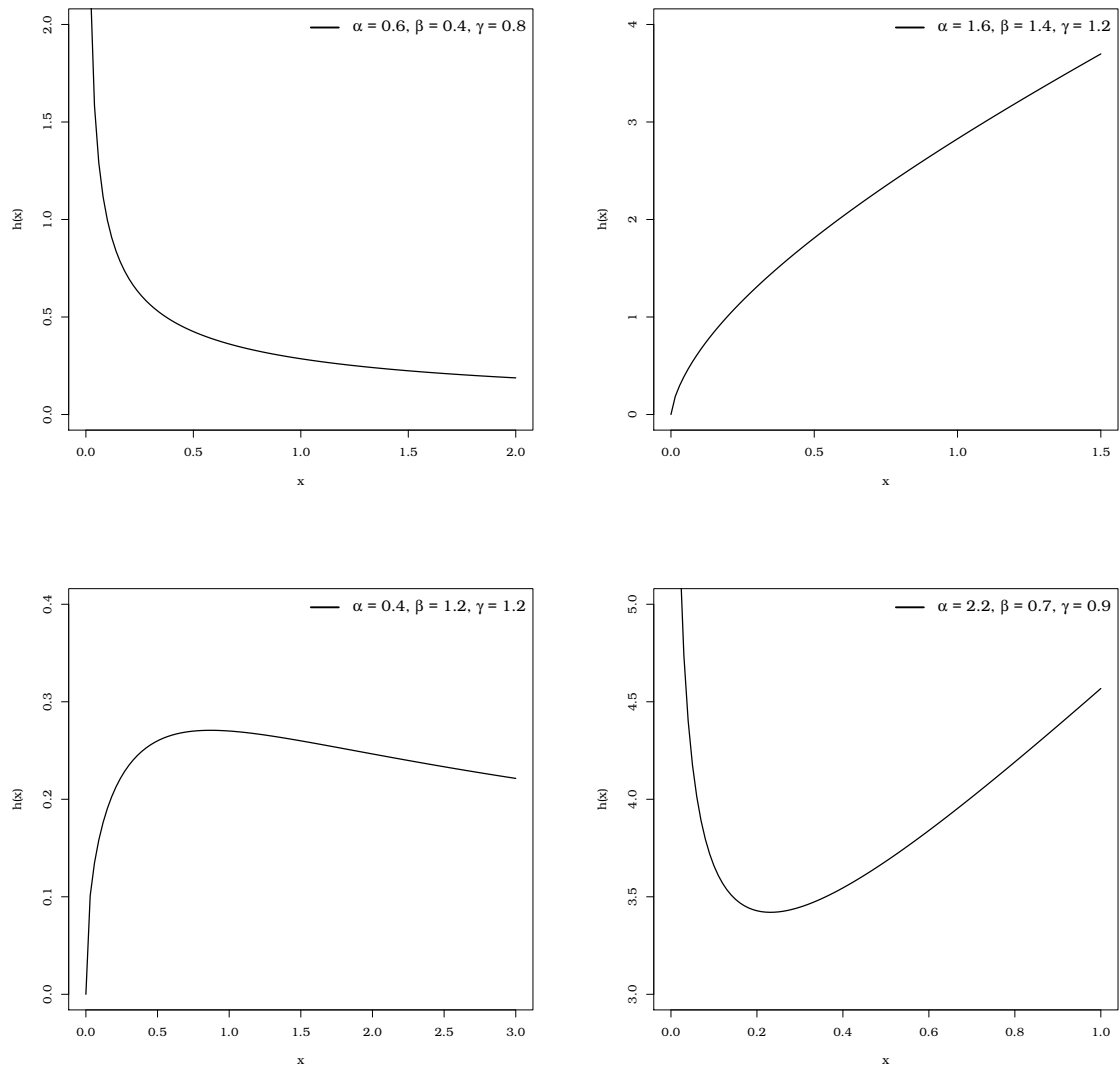
Figure 2.2: Plots of the EGPW hrf for \lambda = 1 .
