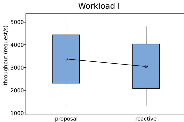
Figure 13 – Boxplot scenario 1.
