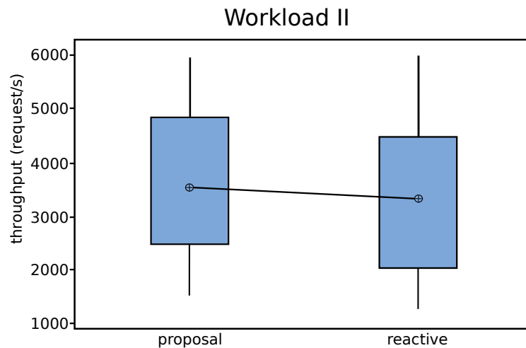
Figure 14 – Boxplot scenario 2.
