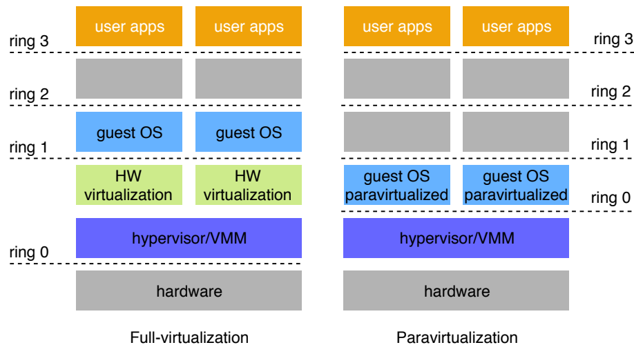
Figure 19 – Virtualization.
