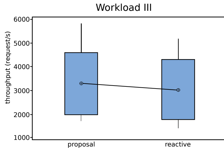
Figure 15 – Boxplot scenario 3.
