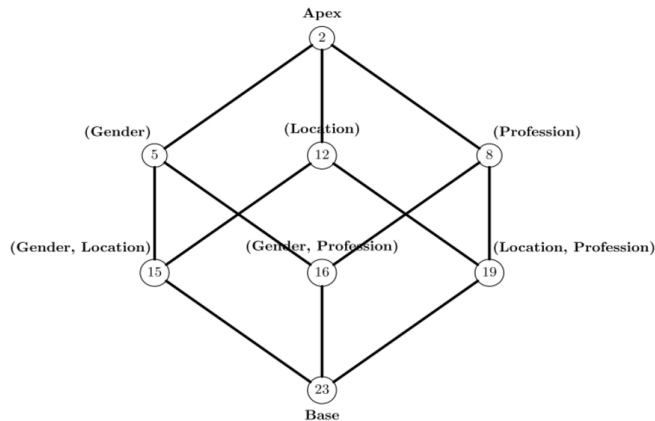
Figure 15 – Graph Cube Lattice
