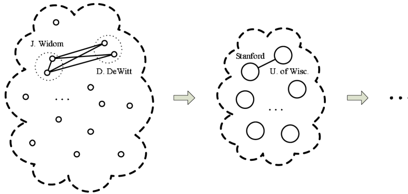
Figure 17 – Example of Topological Aggregate Graph
