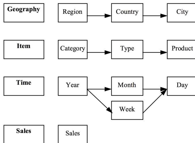
Figure 2 – Example of dimensions and measure for a sales application
