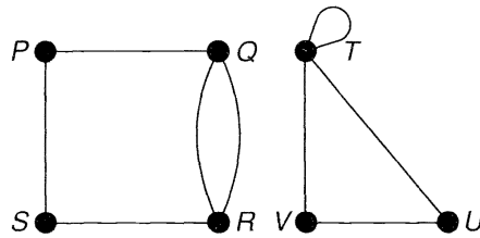
Figure 6 – Example of a multigraph with a loop
