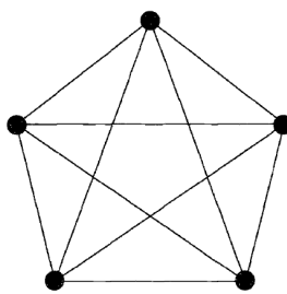
Figure 7 – Example of a complete graph
