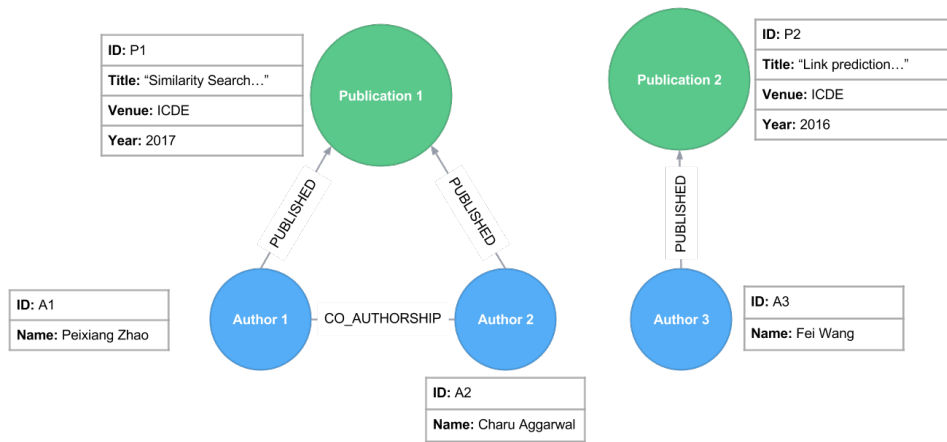
Figure 26 – Schema representation of the DBLP data graph
