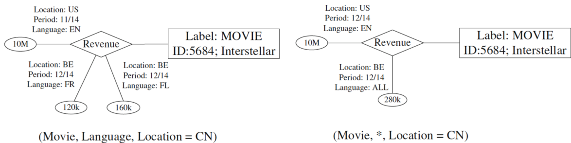
Figure 25 – Aggregate Graph for intra-class dimensionl
