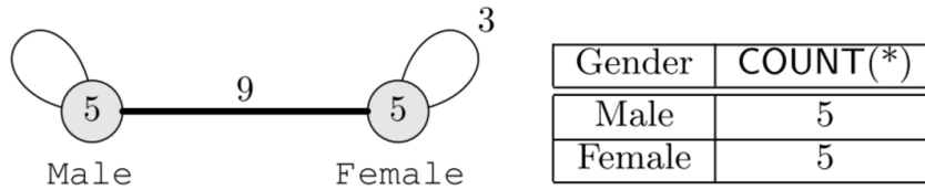
Figure 14 – Aggregate Network by Gender dimension
