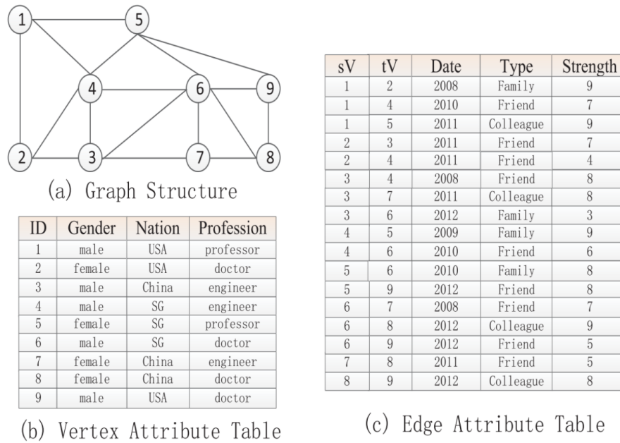
Figure 21 – Example of attributed graph
