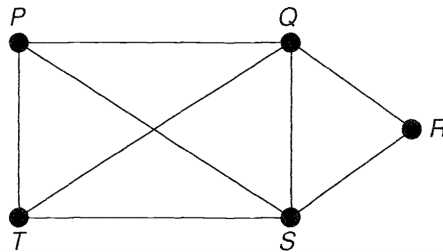
Figure 4 – Example of graph
