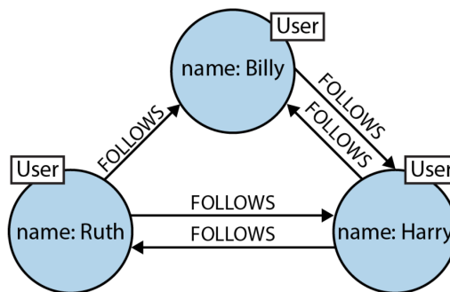
Figure 5 – Example of graph representation of a social network
