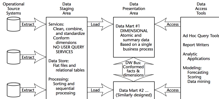
Figure 1 – Elements of a Data Warehouse
