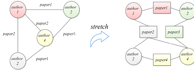
Figure 20 – Example of stretch operation
