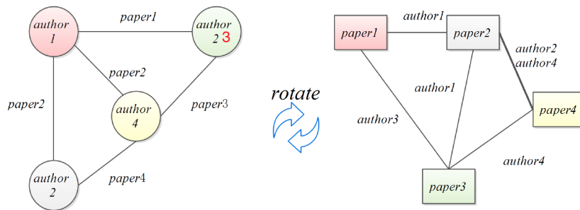
Figure 19 – Example of rotate operation
