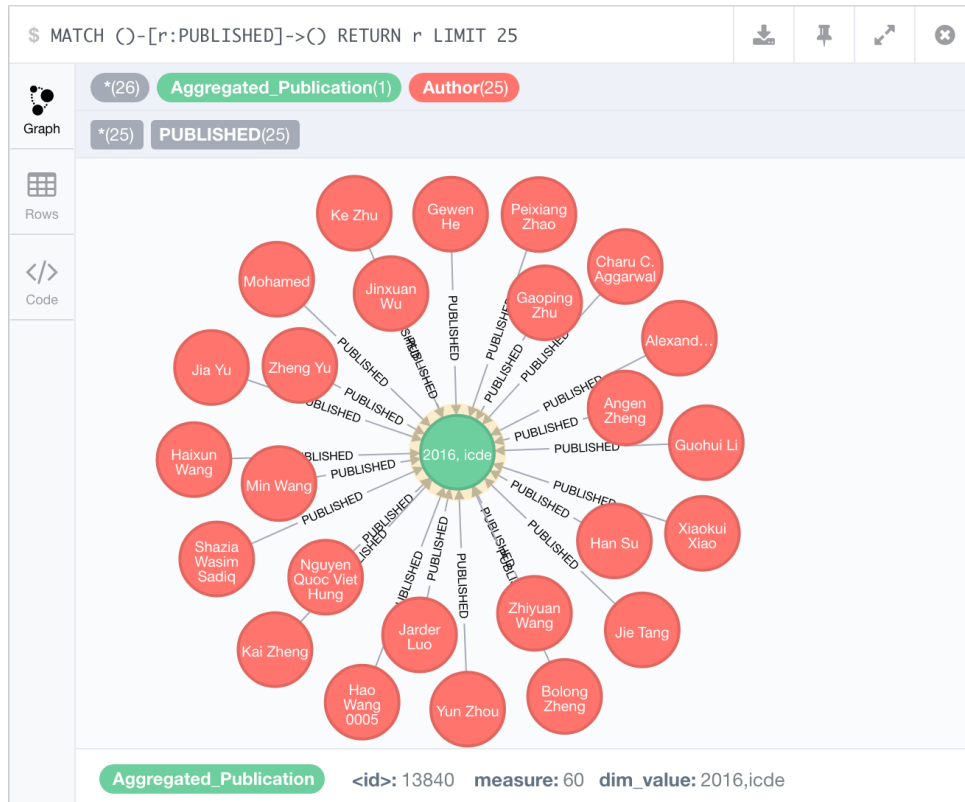
Figure 31 – Subgraph from the Aggregate Graph generated by the GA
