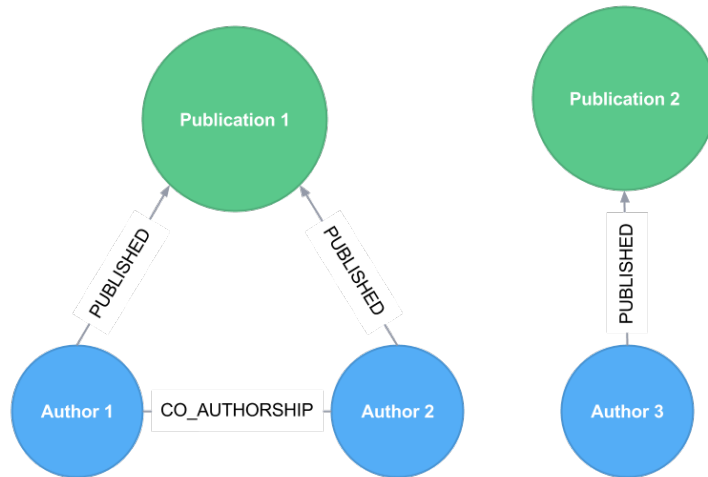
Figure 30 – DBLP dataset schema in graph database
