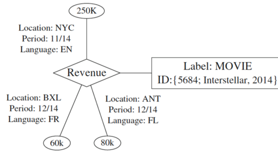
Figure 24 – Movie graph on GRAD model
