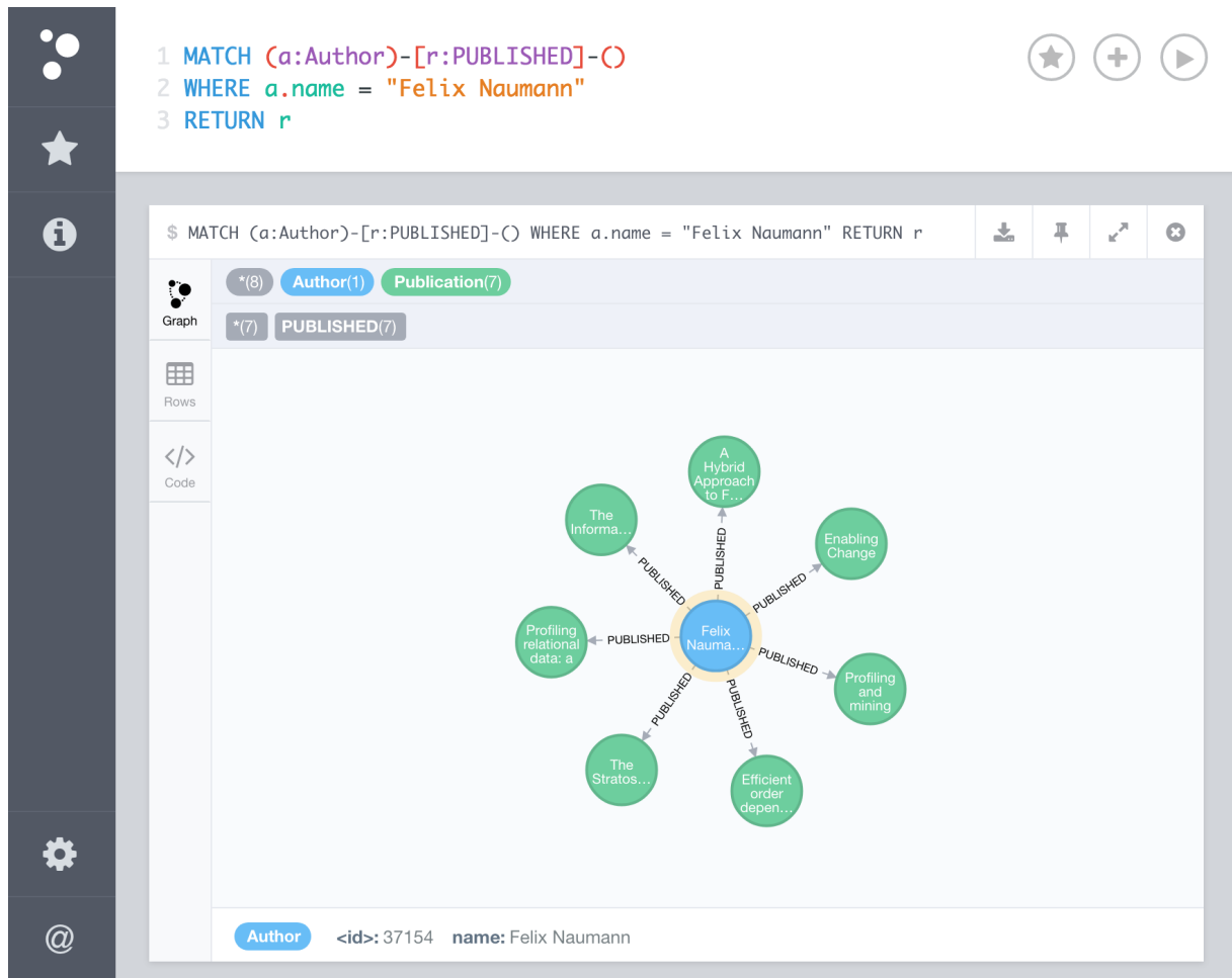
Figure 12 – Neo4J User Interface
