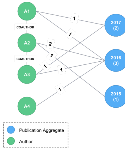
Figure 29 – Aggregate Graph obtained from running example graph
