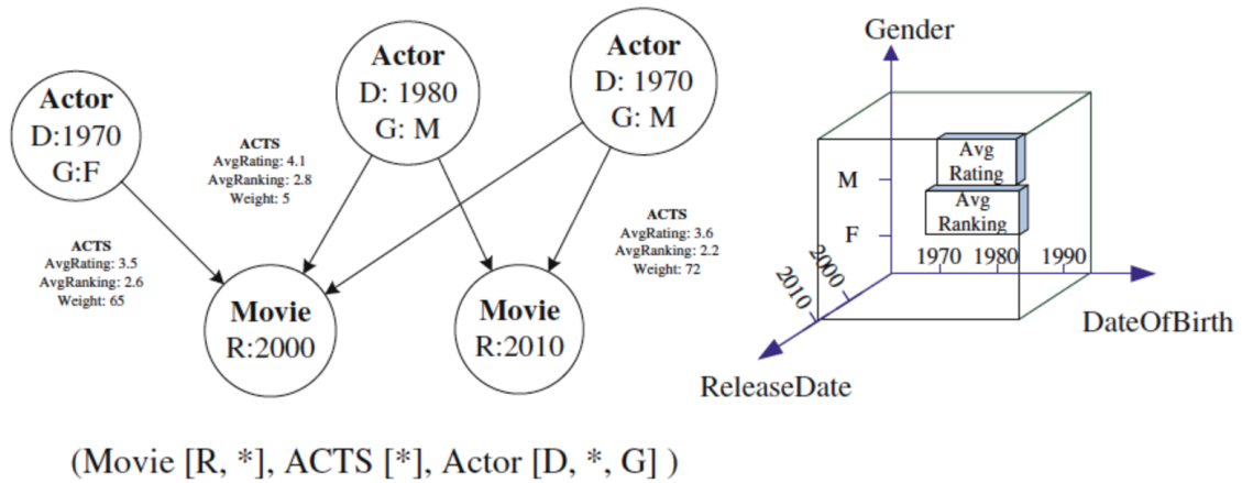
Figure 23 – Aggregate Graph for inter-class dimensions
