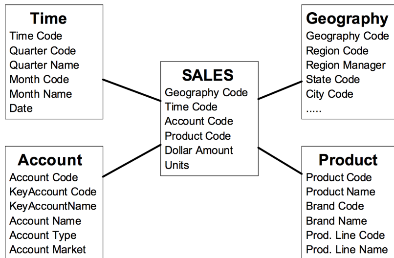
Figure 3 – Example of a Star Schema
