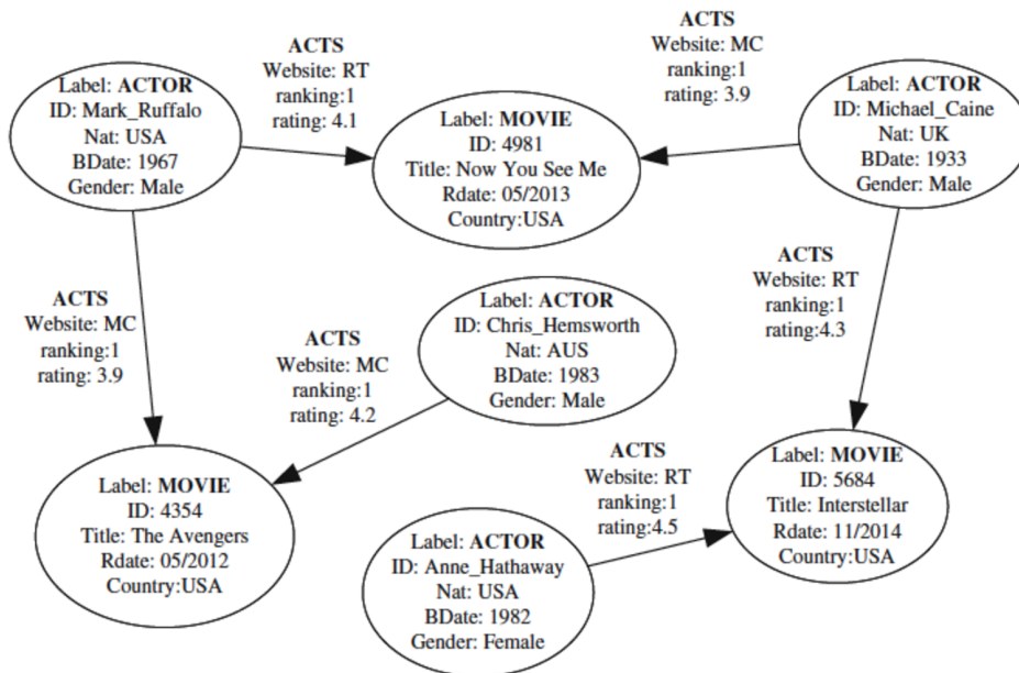
Figure 22 – Original movie graph
