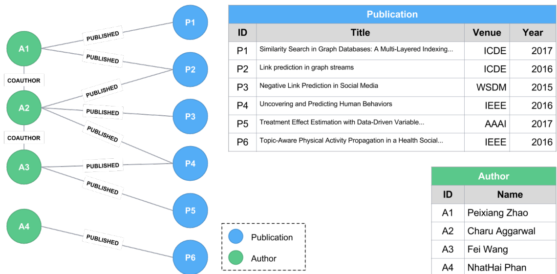
Figure 27 – Running Example with subset of DBLP dataset
