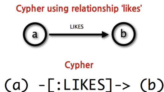
Figure 10 – Cypher syntax representation of a relationship in the graph
