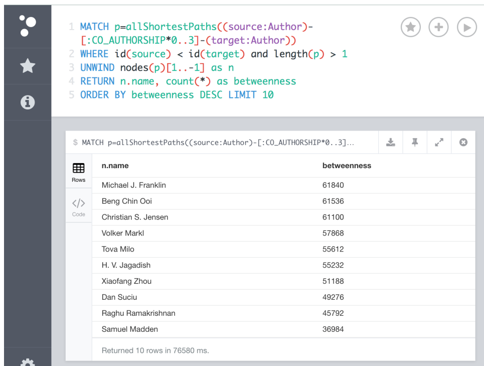
Figure 36 – Result of experiment with the betweenness centrality measure for Authors
