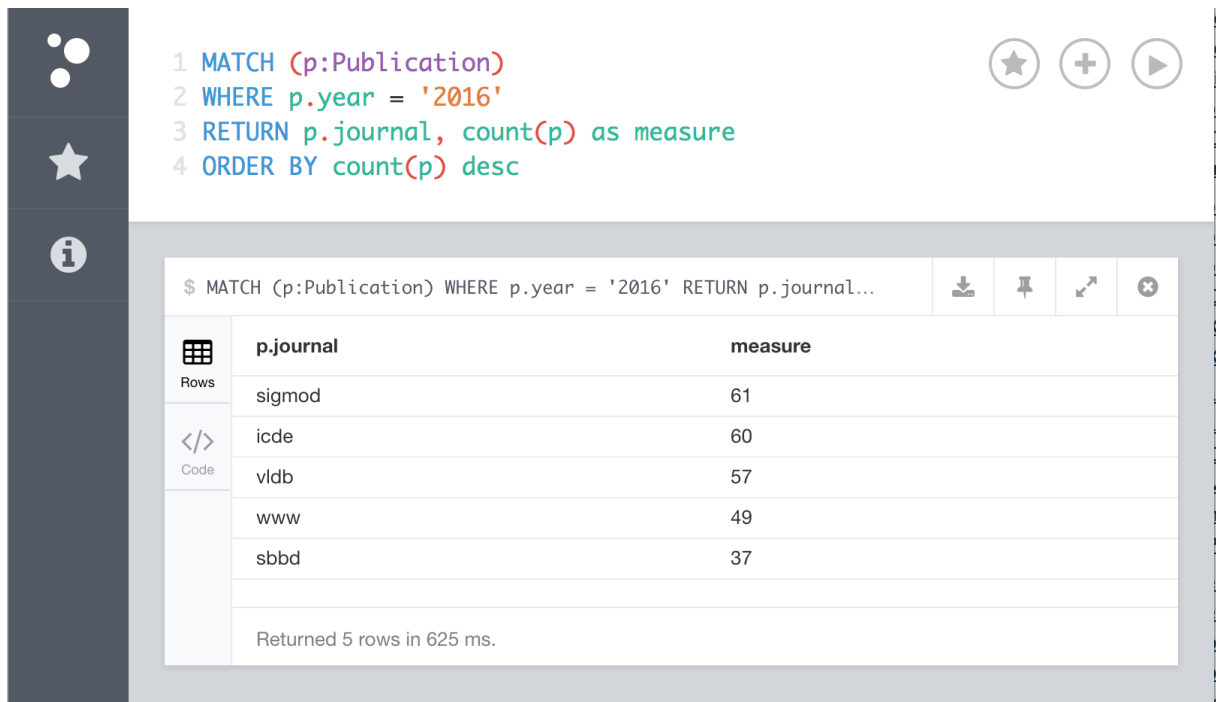
Figure 38 – Result of experiment with content-based measure query submitted to the original graph
