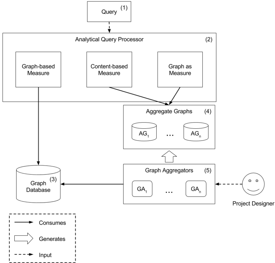
Figure 28 – OLAP Analysis over Graph Databases Architecture
